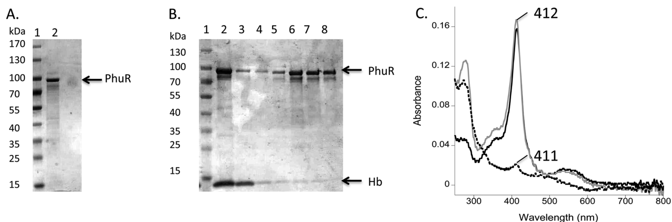
Figure 4. Heme binding properties of PhuR. (A) Apo-PhuR (10 \mu M) following elution from hemin-agarose in SDS loading buffer (50 \mu L). PhuR (10 \mu L) was analyzed on a 12% SDS-PAGE gel. (B) Elution of PhuR (5 \mu M) from Ni-NTA resin following incubation with metHb (4 \mu M). Lane 1, molecular weight markers; Lane 2, apo-PhuR and metHb prior to loading; Lane 3, Ni-NTA flow through; Lane 4, wash in 20 mM Tris-HCl (pH 7.5), 250 mM NaCl, and 5 mM Im; Lane 5, wash in 20 mM Tris-HCl (pH 7.5), 50 mM NaCl, and 20 mM Im; Lanes 6–8, elution fraction in 20 mM Tris-HCl (pH 7.5) containing 50 mM NaCl and 250 mM Im. (C) Spectra of metHb with apo-PhuR in 20 mM Tris-HCl (pH 7.5), 250 mM NaCl, and 5 mM Im (gray solid line), wash fraction in 20 mM Tris-HCl (pH 7.5), 250 mM NaCl, and 5 mM Im (black solid line), and elution fraction in 20 mM Tris-HCl (pH 7.5) containing 50 mM NaCl and 250 mM Im (black dashed line).
