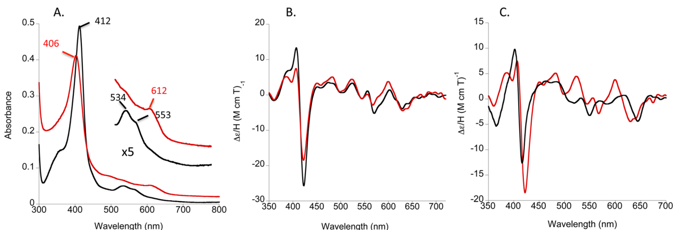
Figure 7. Absorption and MCD spectra of the PhuR Y519A mutant. (A) Absorption spectra of imidazole-coordinated PhuR Y519A (8.5 \mu M) (black line) and following dialysis (red line) at 4 ^{\circ} C in 50 mM Tris-HCl (pH 7.5), 50 mM NaCl, and 0.07% LDAO. (B) MCD spectra of the wild-type (black line) and Y519A (red line) PhuR as in (A). (C) MCD spectra of Fe(III)-Mb (black line) in 50 mM Tris-HCl (pH 7.5), 50 mM NaCl, and Y519A PhuR (red line) under the same conditions as those in (B).
