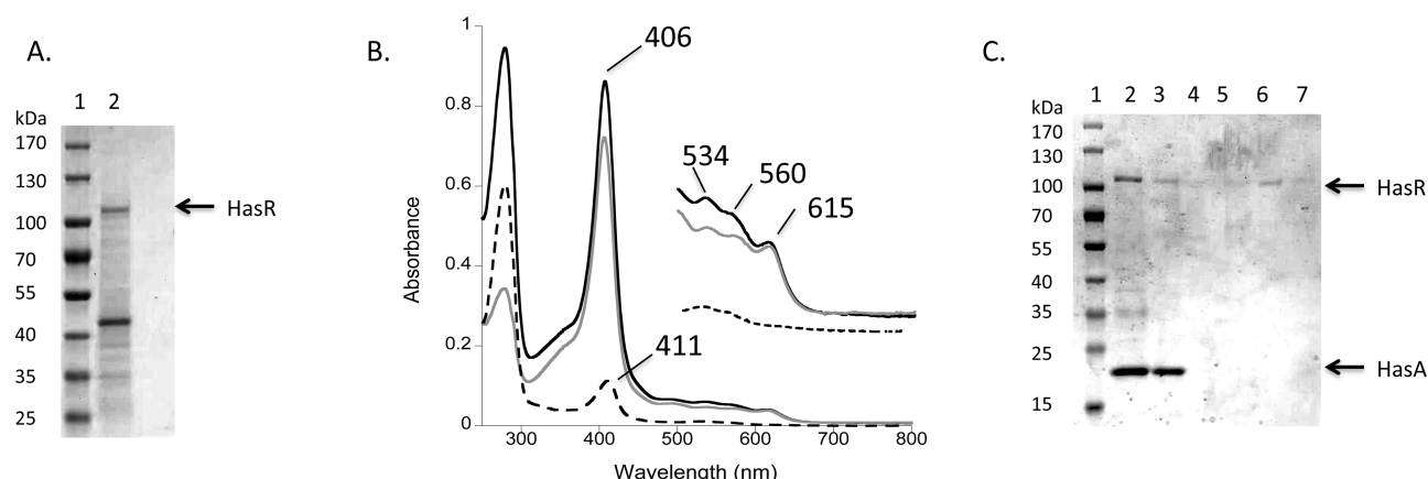
Figure 3. Heme binding properties of purified HasR. (A) Apo-HasR (10 \mu M) following elution from hemin-agarose in SDS-loading buffer (50 \mu L). HasR (10 \mu L) was analyzed on a 12% SDS-PAGE gel. (B) Spectra of 5 \mu M apo-HasR (black dashed line) prior to incubation with holo-HasA, 4 \mu M holo-HasA (gray solid line), holo-HasA, and apo-PhuR following incubation (black solid line). Inset: 5 \times magnification of the visible region, 500–800 nm. (C) Elution of HasR (5 \mu M) from Ni-NTA resin following incubation with HasA (4 \mu M). Lane 1, molecular weight markers; Lane 2, Ni-NTA flow through; Lane 3, wash in 20 mM Tris-HCl (pH 7.5), 250 mM NaCl, and 5 mM Im; Lane 4, wash in 20 mM Tris-HCl (pH 7.5), 50 mM NaCl, and 20 mM Im; Lanes 5–7, elution in 20 mM Tris-HCl (pH 7.5) containing 50 mM NaCl and 250 mM Im.
