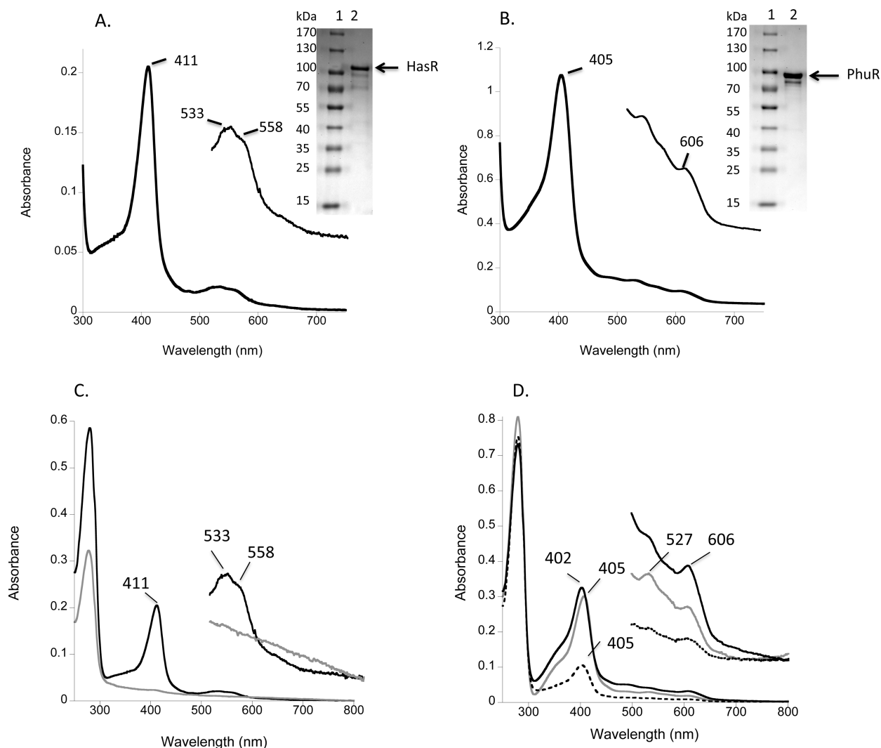
Figure 2. Purification of HasR and PhuR from cultures supplemented with heme or Hb. (A) Absorption spectrum of the purified partially heme-loaded Fe(III) holo-HasR receptor (5 \mu M). Inset: SDS-PAGE of purified HasR. Lane 1, molecular weight markers; Lane 2, 10 \mu g of purified HasR. (B) Absorption spectrum of the purified partially heme loaded PhuR receptor (20 \mu M). Inset: SDS-PAGE of purified PhuR. Lane 1, molecular weight markers; Lane 2, 10 \mu g of purified HasR. (C) Spectra of HasR purified from cultures supplemented with (black line) or without (gray line) 10 \mu M heme. (D) PhuR purified from nonsupplemented cultures (black dashed line), cultures supplemented with 10 \mu M heme (gray solid line), or cultures supplemented with 10 \mu M Hb (black solid line). All visible region 500–800 nm insets were magnified 5 \times .
