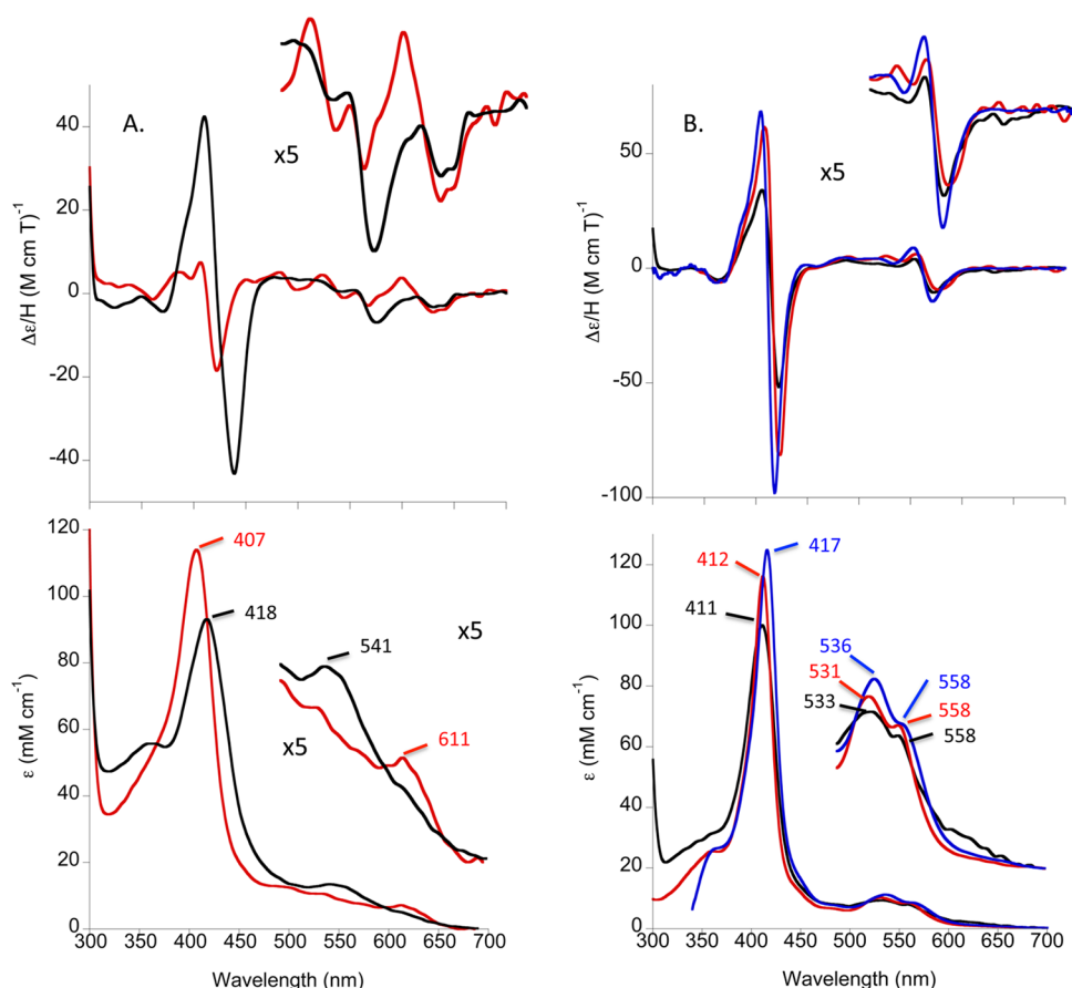
Figure 8. Absorption and MCD spectra of the PhuR Y519A and Y519H mutants. (A) Absorption (lower panel) and MCD (upper panel) of PhuR Y519A (red line) and Y519A-CN (aliquots of 1 mM KCN until apparent saturation) (black line) at 4 ^{\circ} C in 50 mM Tris-HCl (pH 7.5), 50 mM NaCl, and 0.07% LDAO. (B) Absorption and MCD spectra of PhuR Y519H (black line), Fe(III) Cytochrome b_5 (red line), and Fe(III) Mb H93G-bis-Im complex (1 mM Im) (blue line) in 50 mM Tris-HCl (pH 7.5), 50 mM NaCl. The Fe(III) Mb H93G-bis-Im complex spectrum was replotted from ref 42. Copyright 2011 American Chemical Society.
