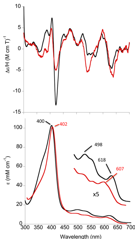
Figure 9. Absorption and MCD spectra of the PhuR H124A mutant. Absorption (lower panel) and MCD (upper panel) of PhuR H124A (red line) and holo-ShuT (black line) at 4 °C in 50 mM Tris-HCl (pH 7.5), 50 mM NaCl, and 0.07% LDAO in the case of the PhuR H124A receptor.
